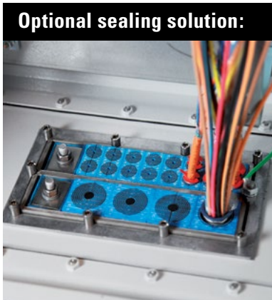
Roxtec CF EMC
