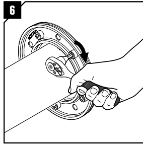
Tighten the bolts crosswise in small steps. Full compression is achieved when the rubber is flush or slightly raised from the steel casing. Do not exceed the maximum torque according to the table on previous page.
