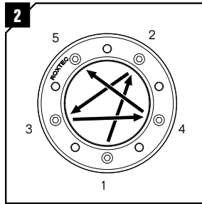
Untighten the bolts crosswise in quarter turn increments.
