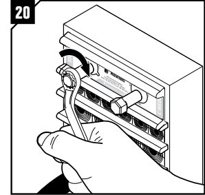
Tighten the screws alternately until full mechanical stop, approx 20 full revolutions per screw. Do not exceed 20 Nm (15 ft.lb.).
