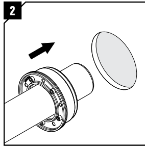
Insert the pipe and seal in the aperture.
