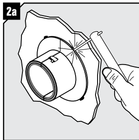
2a Tack weld the fire penetration seal to the structure. Minimum 4 positions.
