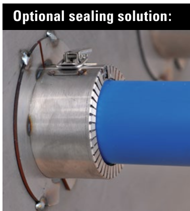
Roxtec Sleeve-it™ Fire penetration seal
