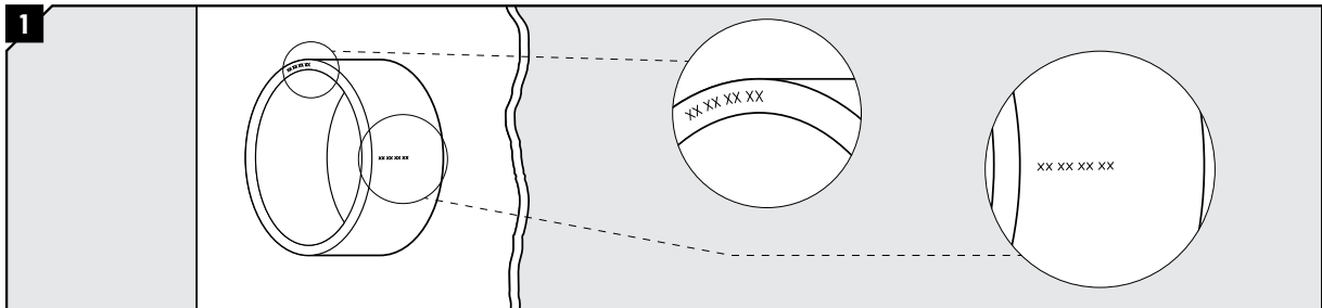
Original Roxtec sleeves are identified by Roxtec marking, serial number marking or label. Sleeves can have marking on the front face or the side.
