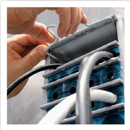
Stayplate clip
