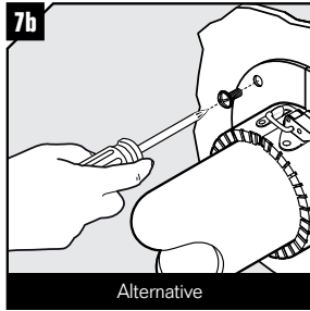
7b Alternative Drill holes in the flange and bolt the fire penetration seal to the structure. Minimum 4 positions.
