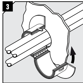
3 Apply the fire penetration seal onto the pipes.
