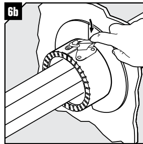
6b Fire penetration seal locked (for larger sizes).
