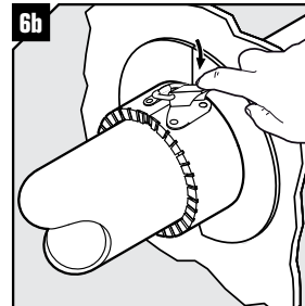
6b Push down the lever to lock the fastener (for larger sizes).
