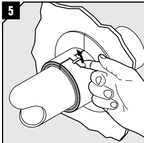
5 Lock the fire penetration seal by pulling the tab over.
