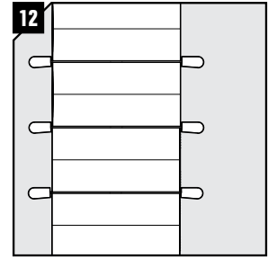
Ensure that the modules are secured within the stayplate edges.
