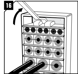
If there is not enough room for the wedge, insert the optional Roxtec pre-compression tool.
