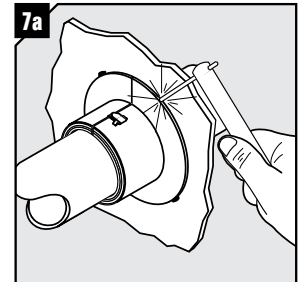
7a Tack weld the fire penetration seal to the structure. Minimum 4 positions.
