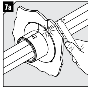
7a Tack weld the fire penetration seal to the structure. Minimum 4 positions.
