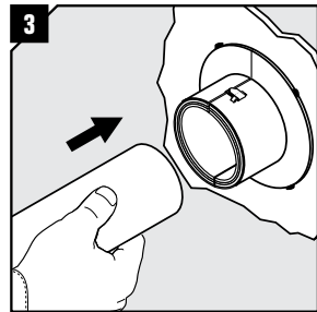
3 Route the pipe through the aperture and fire penetration seal.
