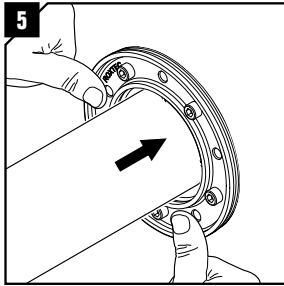
Make sure the seal is properly fitted against the inside of the opening.
